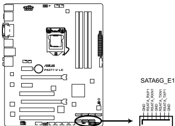
P8277-V LE Marvell® SATA 6.0 Gb/s connectors
