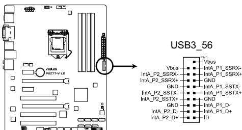
P8Z77-V LE USB3.0 Front panel connector
