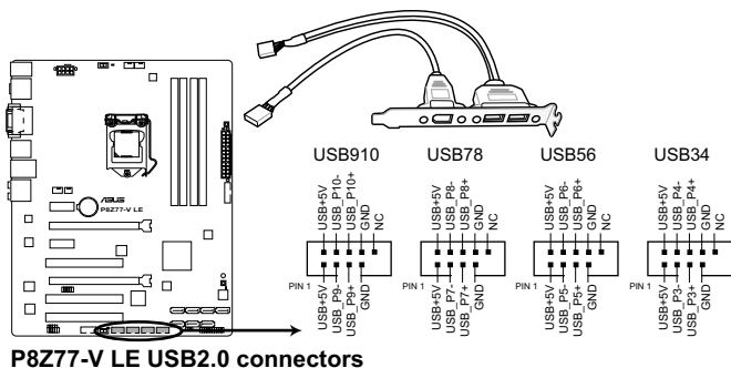
P8277-V LE USB2.0 connectors
