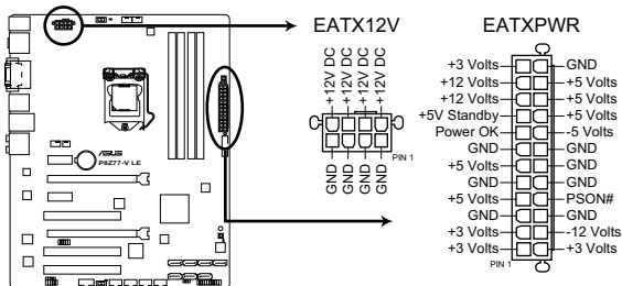
P8277-V LE EATX power connectors
