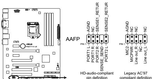
P8277-V LE Front panel audio connector
